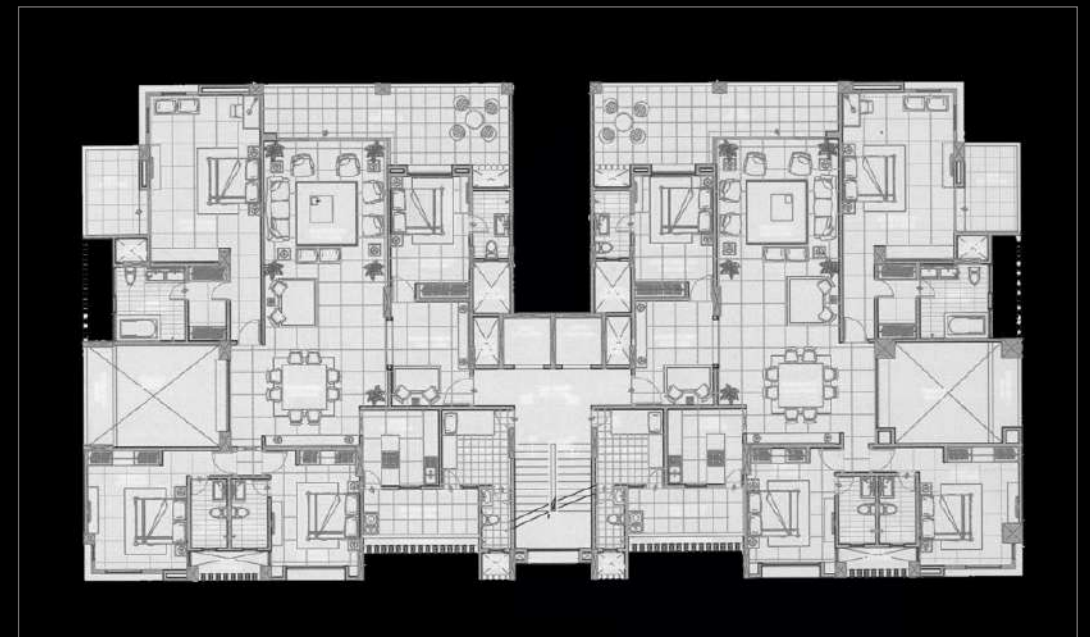
FLOOR PLAN
